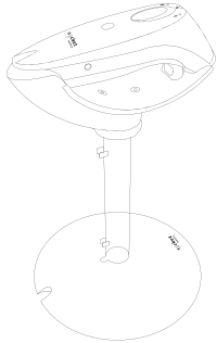
Charging Stand
